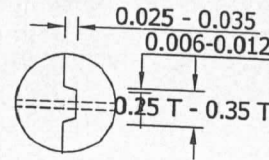
DETIAL A
