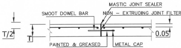
EXPANSION JOINT
