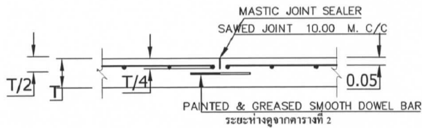
CONTRACTION JOINT
