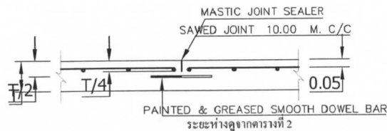
CONTRACTION JOINT
