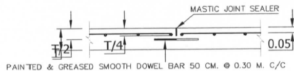
CONSTRUCTION JOINT
